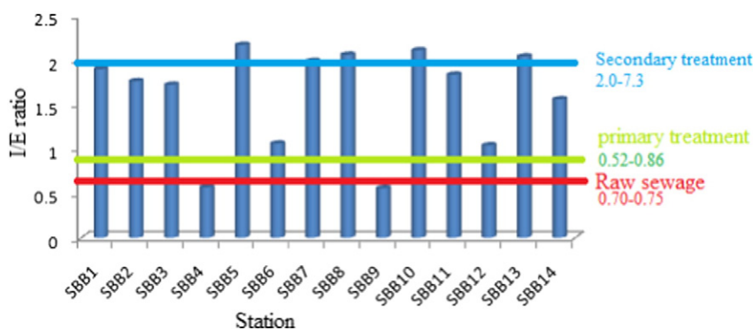
Fig. 3. The I/E ratio in Brunei Bay samples (the horizontal lines are stated as in Takada and Eganhouse, 1998).
