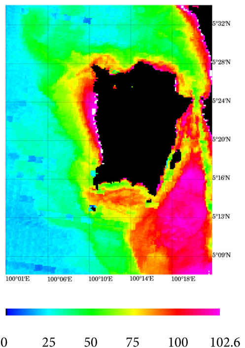
Fig. 4. TSS map generated based on the developed algorithm for the date of 8 December 2009.
