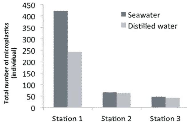
Fig. 5: Proportion of microplastics tested with two different density solutions; saltwater and distilled water
