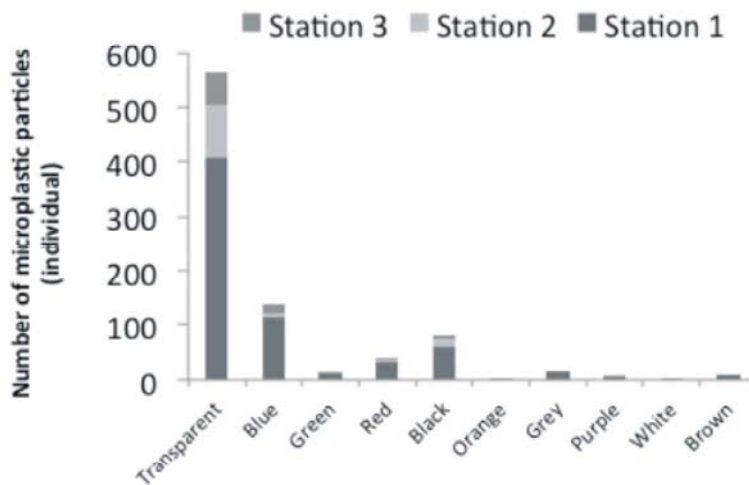
Fig. 4: Amount of microplastics particles found in three stations based on its color
